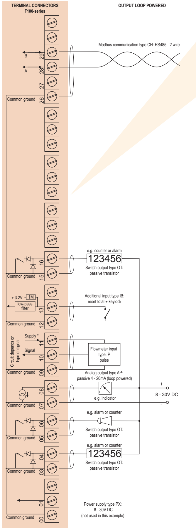
Typical wiring diagram F113-P-AP-CH-IB-OT-(PX)
