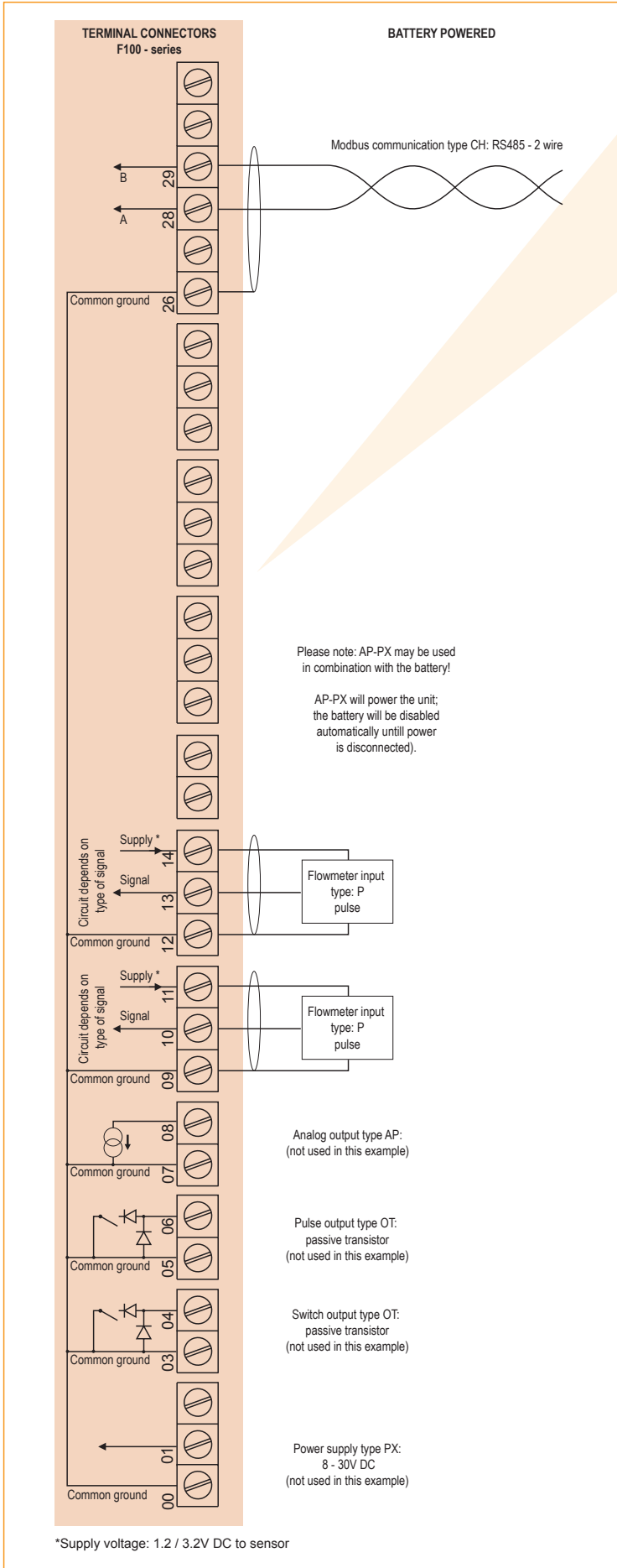
Typical wiring diagram F115-P-(AP)-CH-(OT)-PB-(PX)
