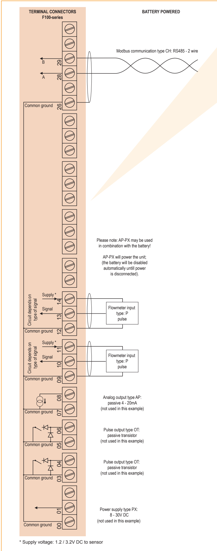
Typical wiring diagram F116-P-(AP)-CH-(OT)-PB-(PX)
