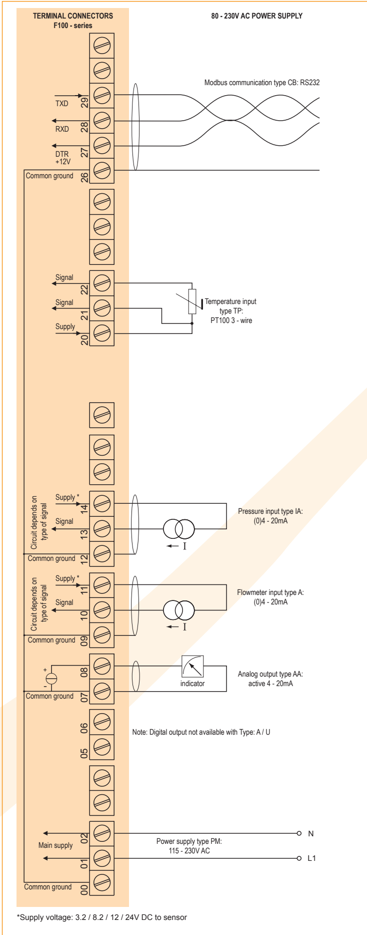
Typical wiring diagram F126-A-AA-CB-EG-IA-OX-PM-TP
