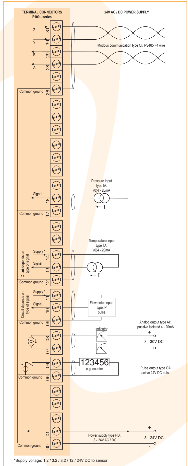
Typical wiring diagram F126-P-AI-CI-EG-IA-OA-PD-TA
