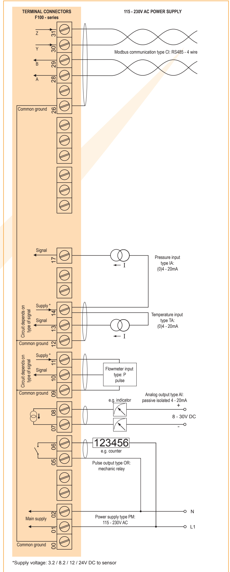
Typical wiring diagram F126-P-AI-CI-EG-IA-OR-PM-TA
