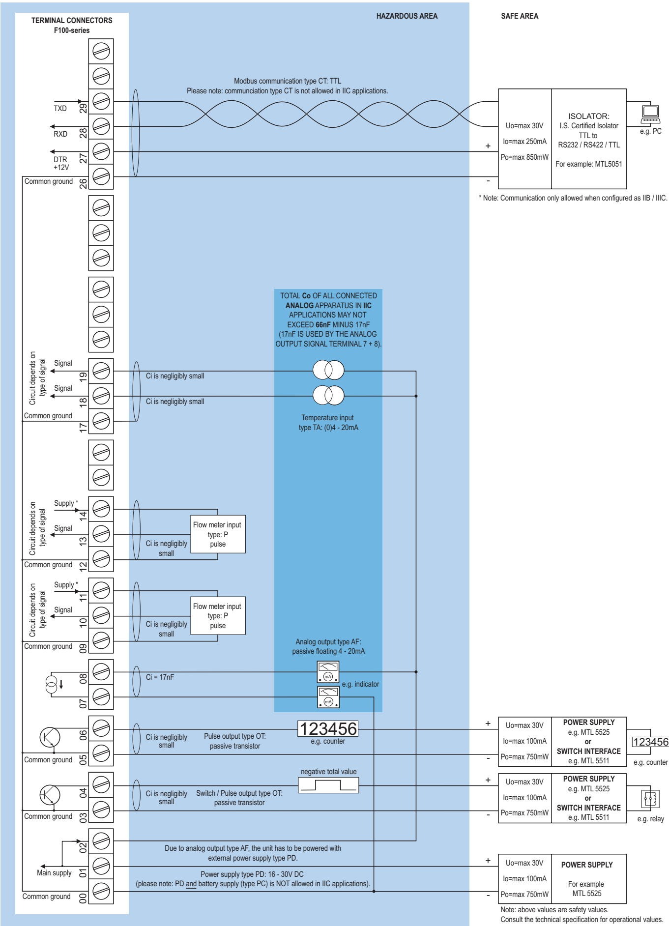
Configuration example IIB / IIC and IIC - F127-P-AF-CT-EL-OT-PD-TA-XI - Power requirement 16 - 30V DC
