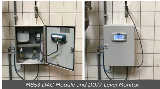
M853 DAC-Module and D077 Level Monitor
