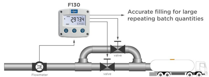
2-stage batch control
