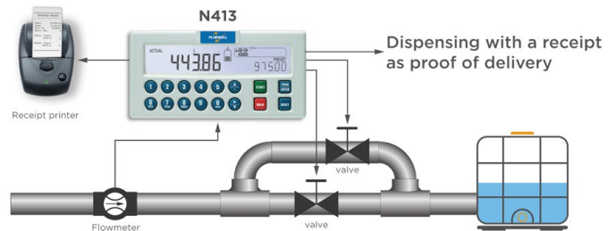
Delivery controller with ticket printer
