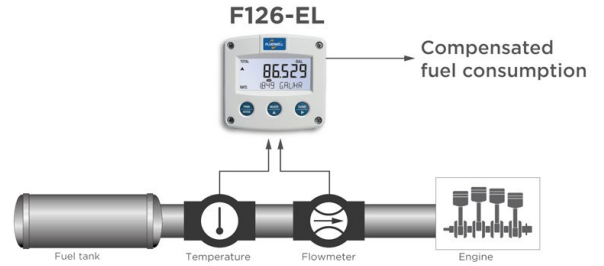
Single line flow measurement with temperature compensation
