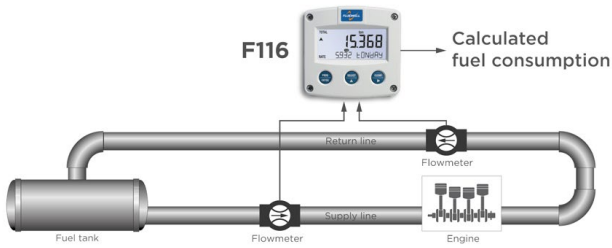
Differential flow measurement
