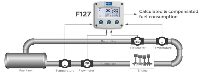
Differential flow measurement with temperature compensation
