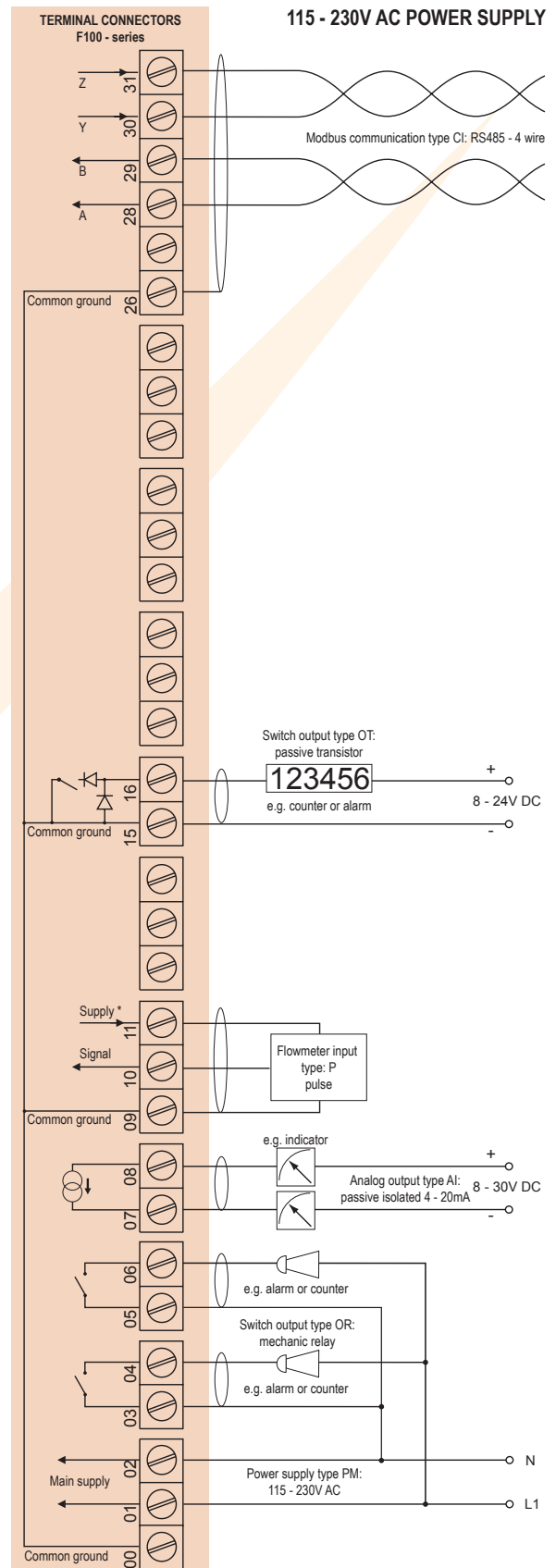
Typical wiring diagram F118-P-AI-CI-OR-PM
