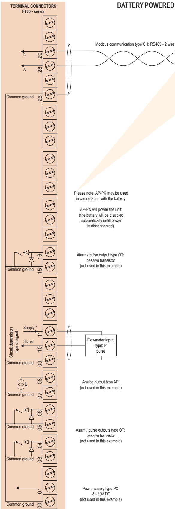
Typical wiring diagram F118-P-(AP)-CH-(OT)-PB-(PX)
