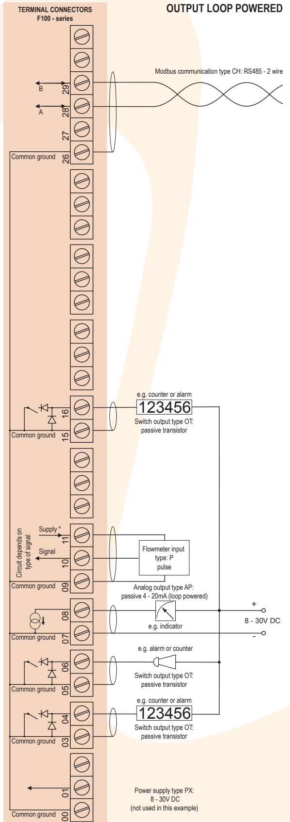
Typical wiring diagram F118-P-AP-CH-OT-PX
