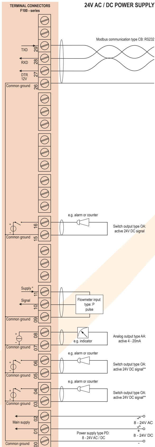
Typical wiring diagram F118-P-AA-CB-OA-PD
