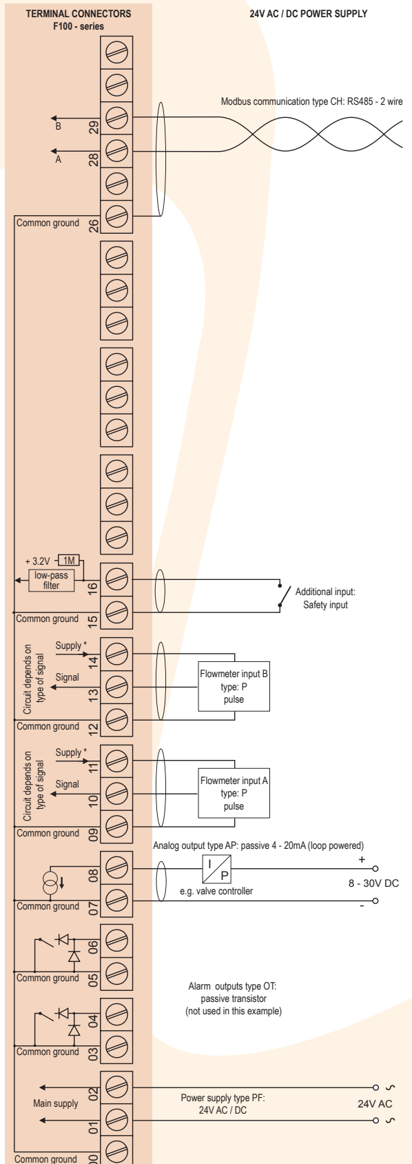
Typical wiring diagram F124-P-AP-CH-PF
