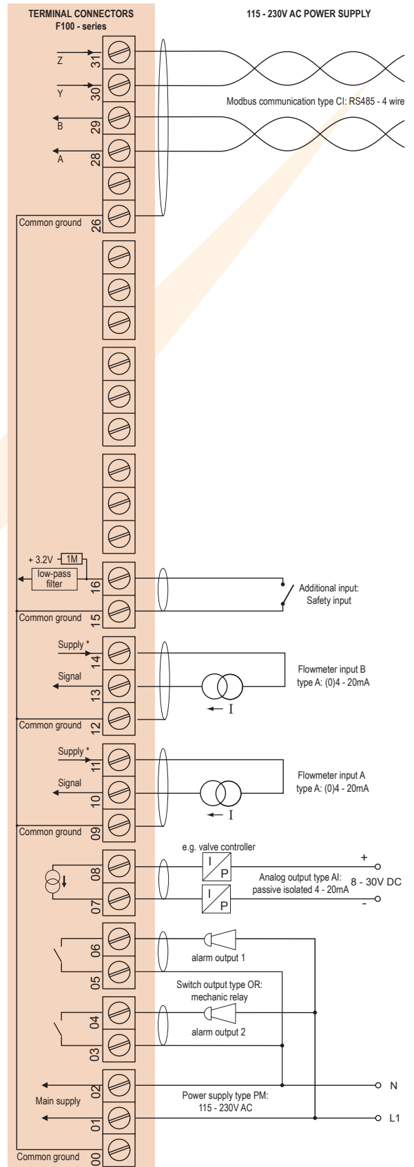
Typical wiring diagram F124-A-AI-CI-OR-PM
