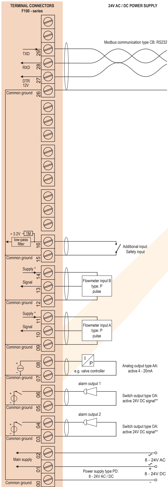
Typical wiring diagram F124-P-AA-CB-OA-PD
